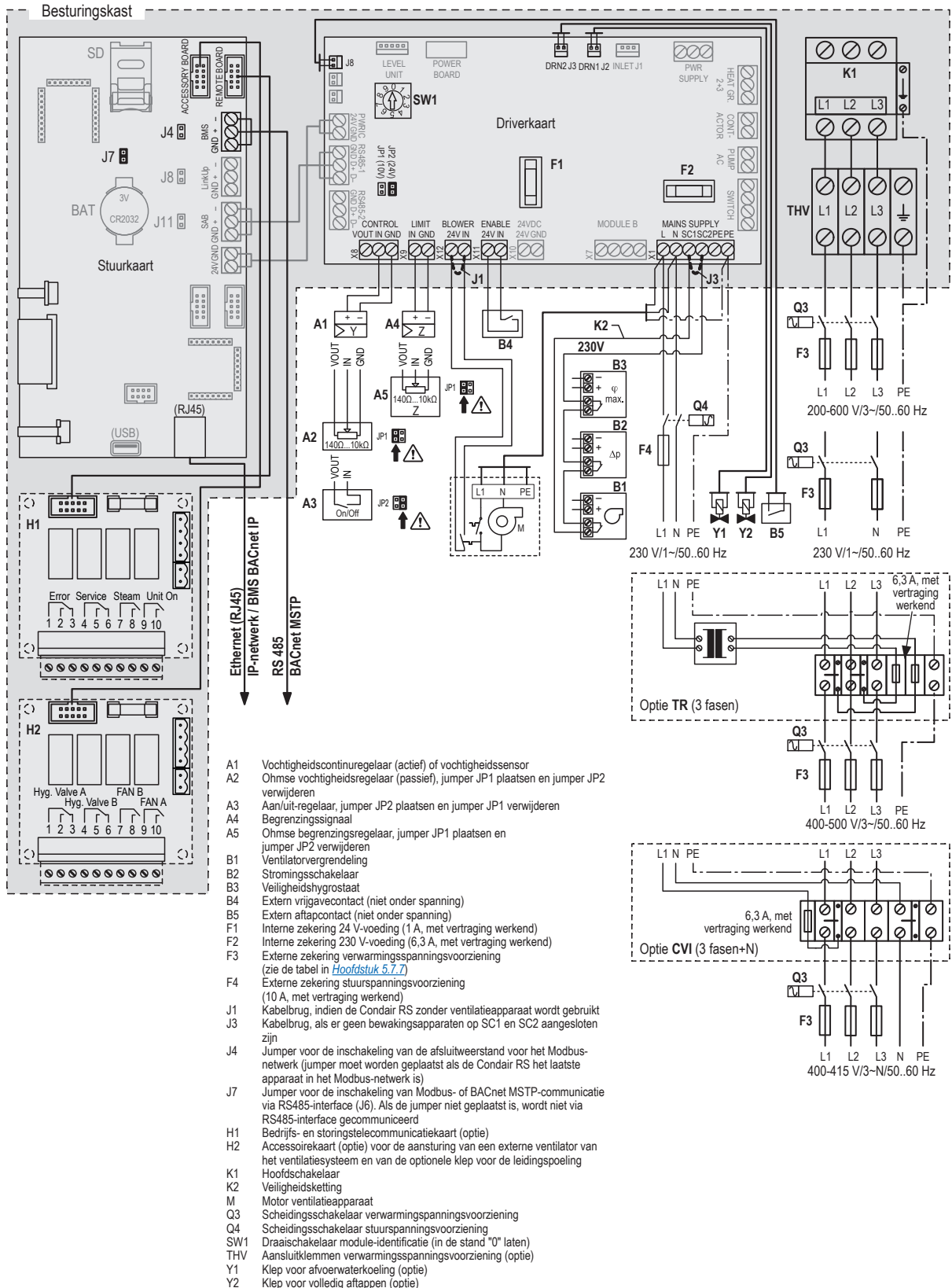
Afb. 27: Elektrisch schema Condair RS 5...40 - stand-aloneapparaten "S" en "M"
