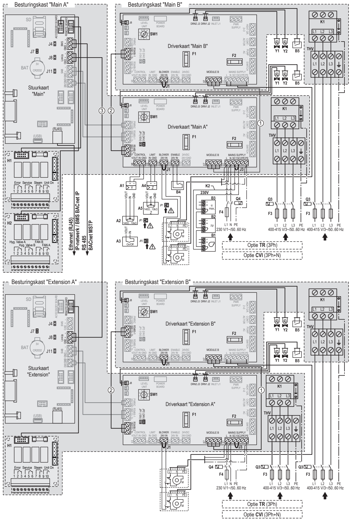
Afb. 30: Elektrisch schema Condair RS 100...160 - Linkup-systemen 3x "M" of 4x "M"
